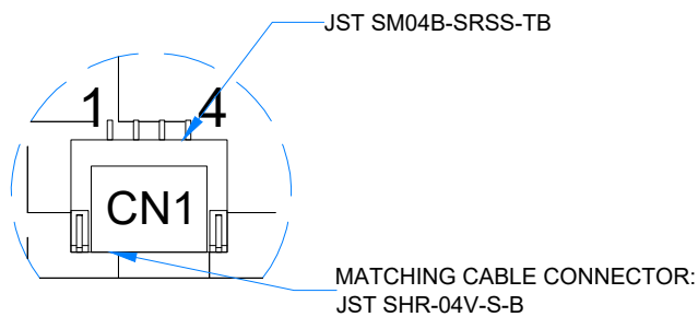
DETAIL B SCALE 4:1
